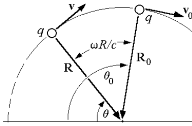
Figure 3. Correlation between the retarded quantities \theta , R and v and the present-time quantities \theta_0 , R_0 and v_0 for a point charge q moving along a circular orbit.
