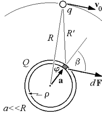
Figure 4. The torque acting on the ring carrying a charge Q and located at the centre of the orbit of q is found by integrating the torque acting on the shaded segment of the ring. Note that the force acting on the shaded sector is in the direction of the velocity vector v_0 of q .
